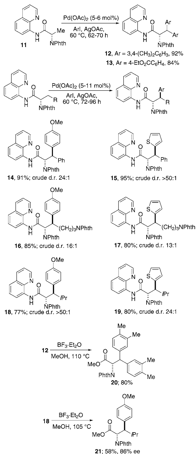
Scheme 3. Aminoquinoline auxiliary.
