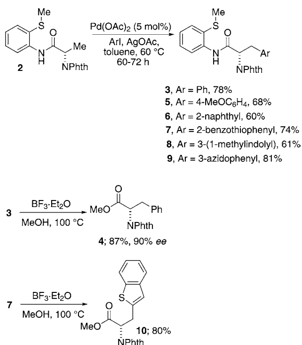
Scheme 2. Synthesis of modified phenylalanine derivatives.
